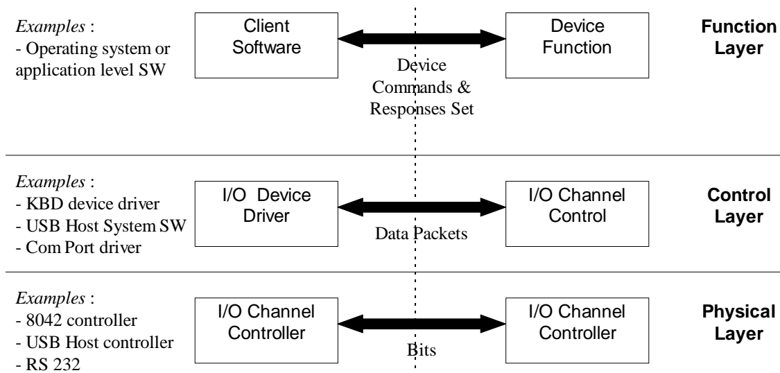
Figure 0-2. Device layers
