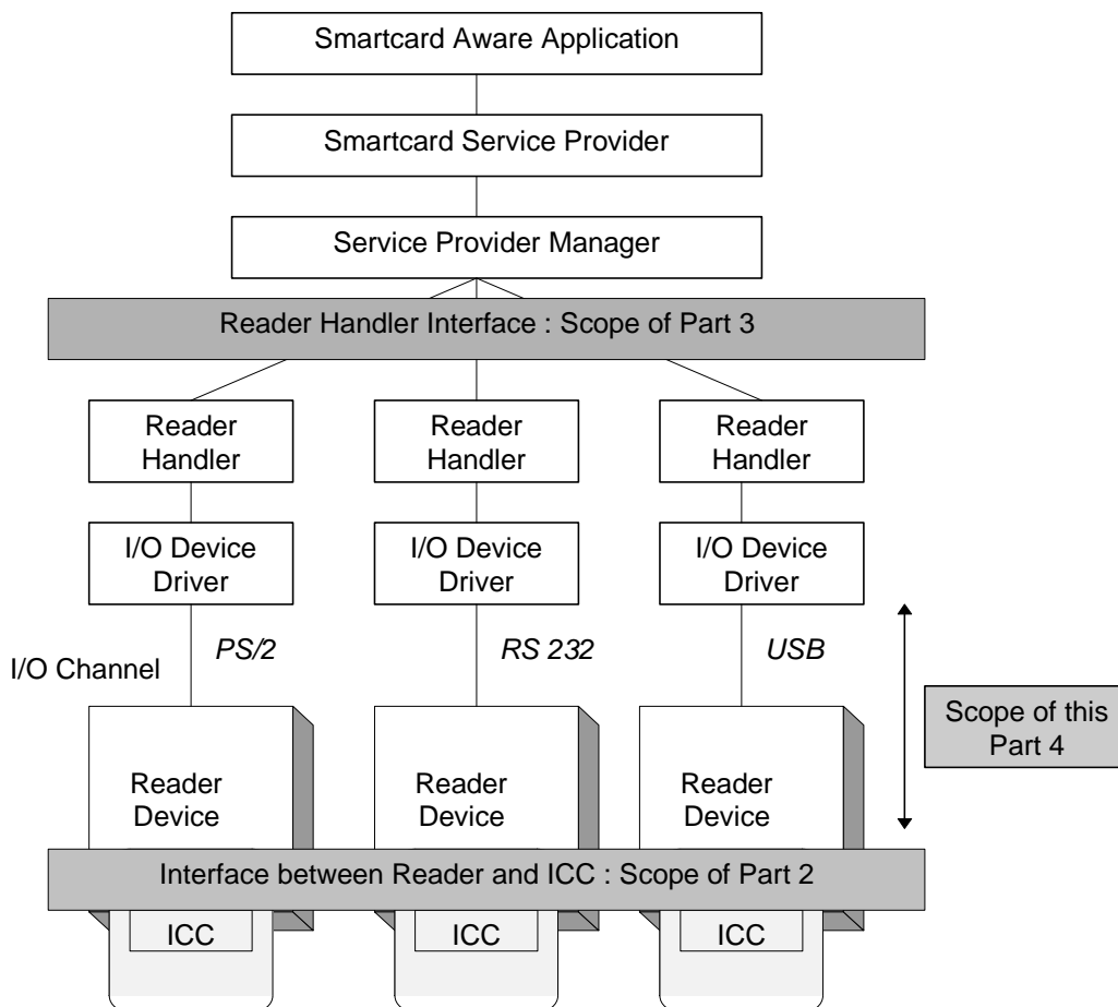
Figure 0-1. IFD Subsystem components and interfaces with other components
