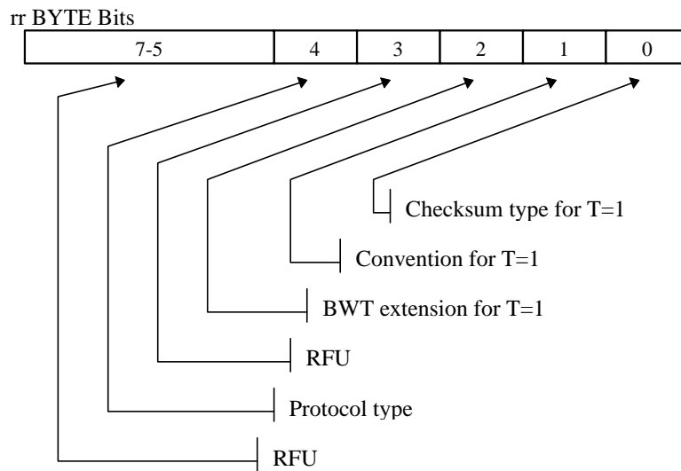
Figure 2-1. rr Byte encoding
