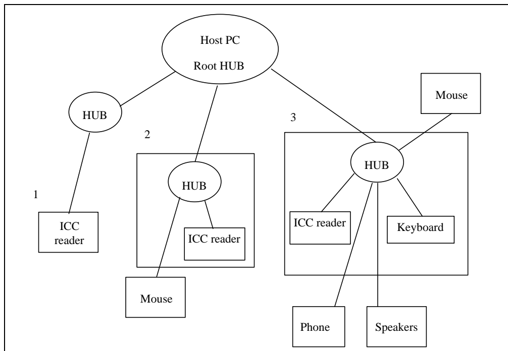
Figure 0-2. Different USB IFD configurations
